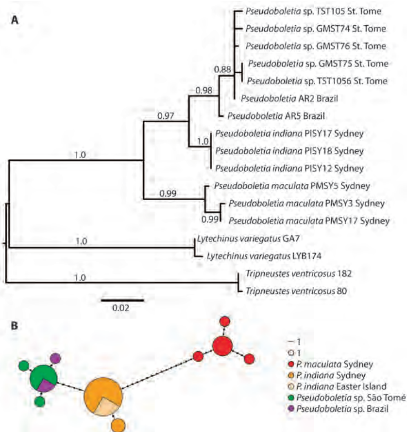
Fig. 5. A. Maximum likelihood tree based on COI sequences (561 pb). Bootstrap score are shown on nodes; B. Haplotype Network.
