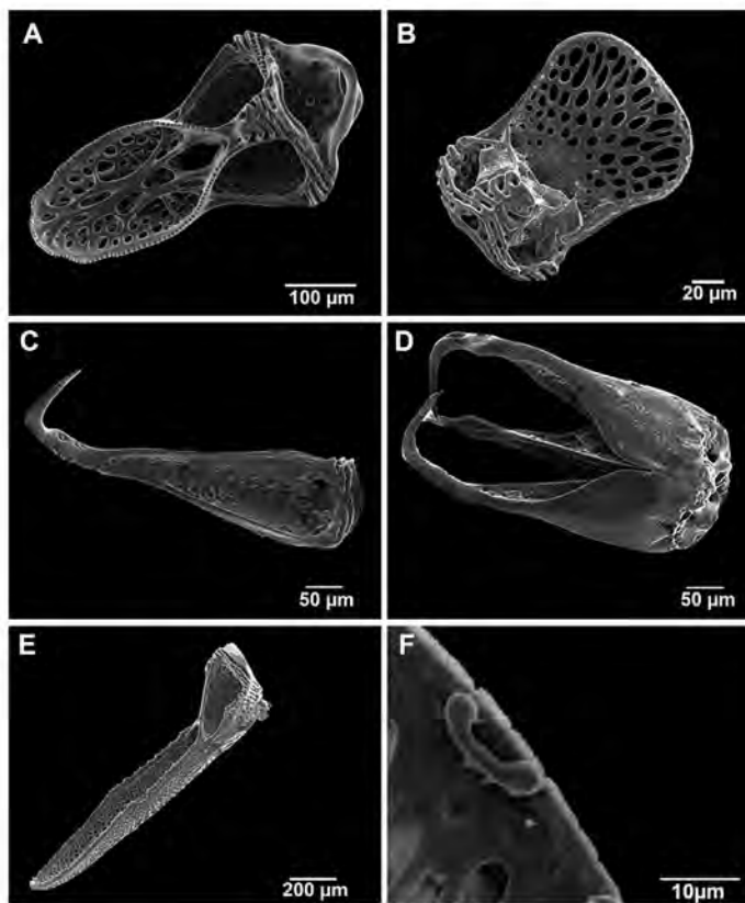
Fig. 3. Morphology of the pedicellariae of Pseudoboletia from Brazil; A. Valve of ophecephalous pedicellaria; B. Valves of triphyllous pedicellaria; C. Valve of globiferous pedicellaria; D. Globifera pedicellaria; E. Valve of tridentate pedicellaria; and F. C-shaped spicule over the skin of the pedicellaria.
