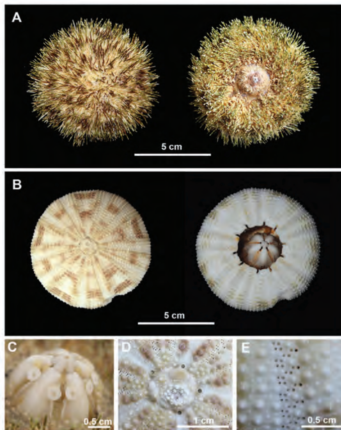
Fig. 2. Morphological details of the Brazilian specimen; A. Aboral and oral view; B. Aboral and oral view of the test; C. Aristotle's lantern in detail showing buccal plates; D. Apical system; and E. Ambulacral regions with four pore-pairs per plate.
