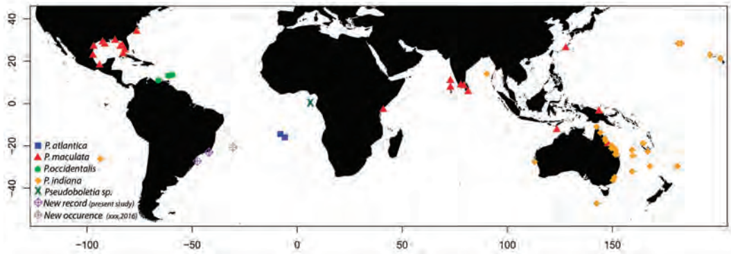
Fig. 4. Distribution of Pseudoboletia species based on the Ocean Biogeographic Information System (OBIS) database, Zigler et al. (2012), Mortensen (1943) and new registers (present study & Martins et al., 2016).
